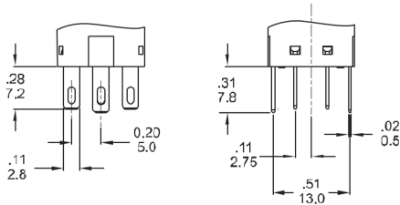
J Solder terminal (std)
