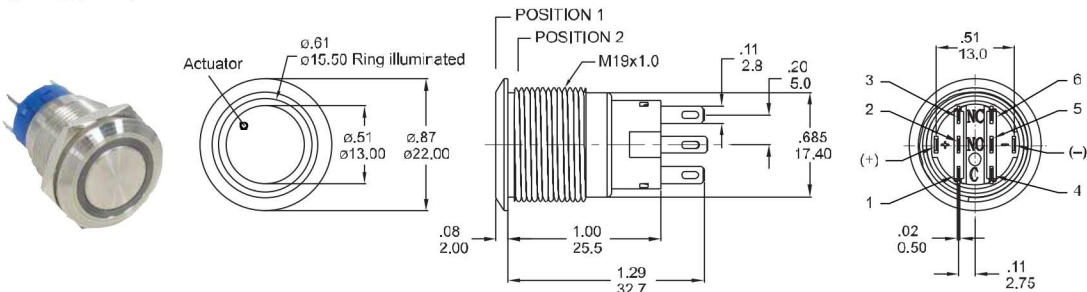
Part No. Shown : MPB19-A0F2□□-JQ
