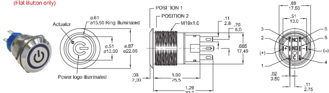
Part No. Shown : MPB19-D0F2□□-JQ
