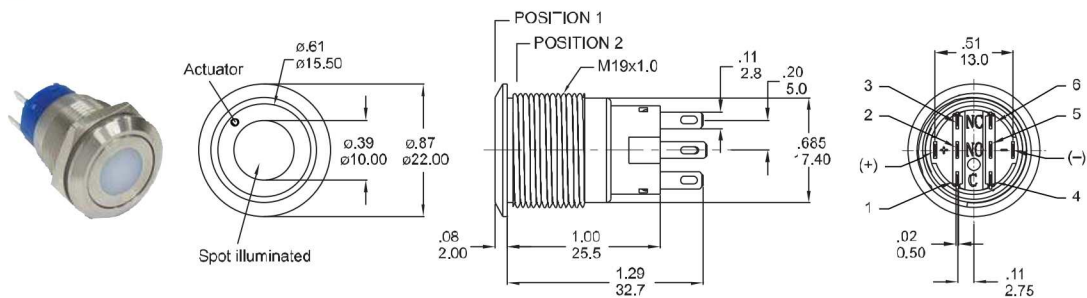
Part No. Shown : MPB19-A0F2□□-JQ
