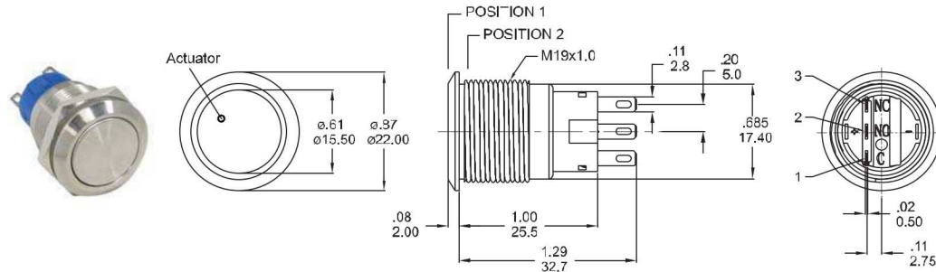
Part No. Shown : MPB19-A0F1□□-JQ
