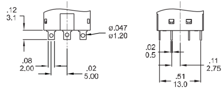
S2 Short solder terminal
